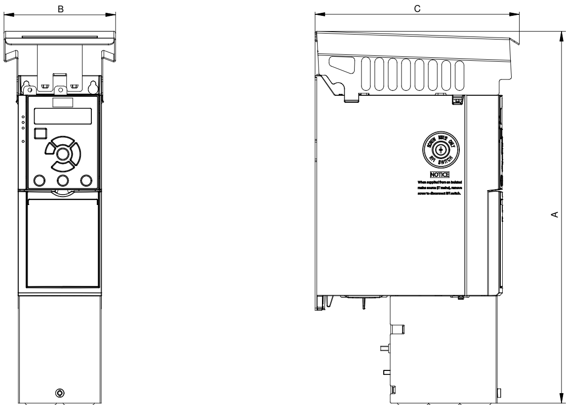
Illustration 18: Standard with IP21/UL/Type 1 kit
