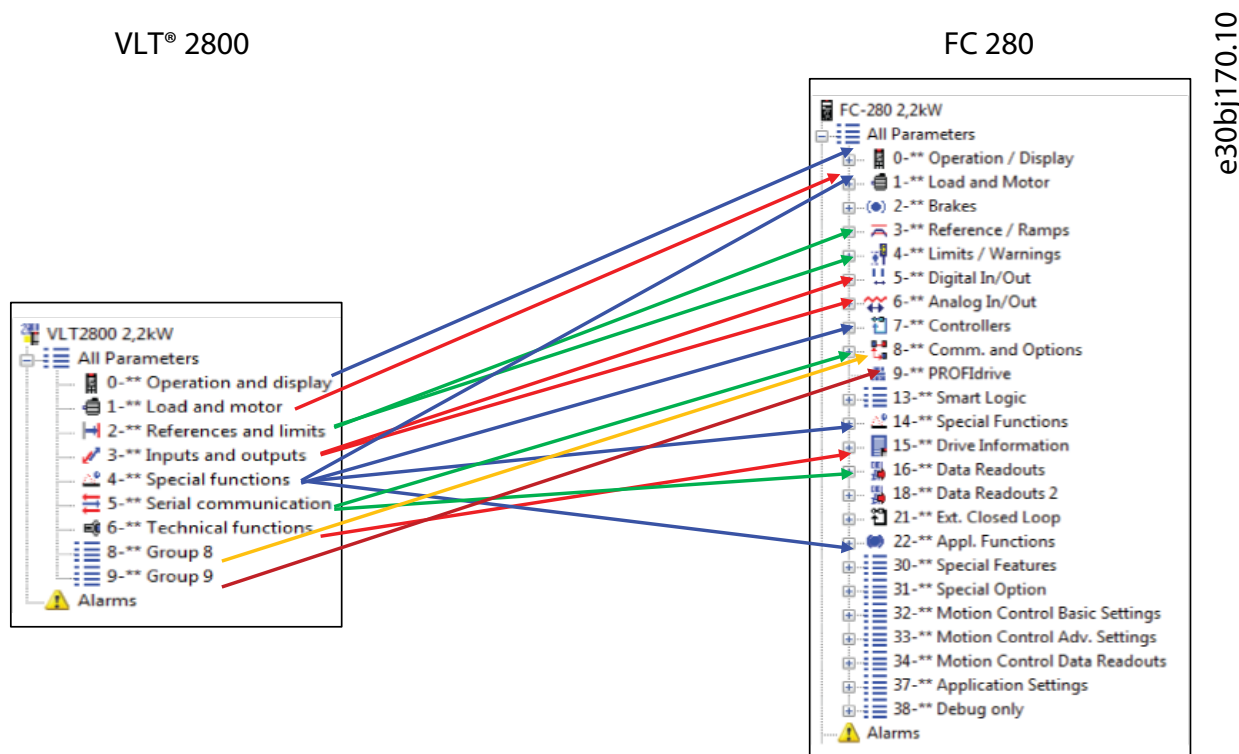
Illustration 54: Corresponding Parameter Groups Between the 2 Drive Series
